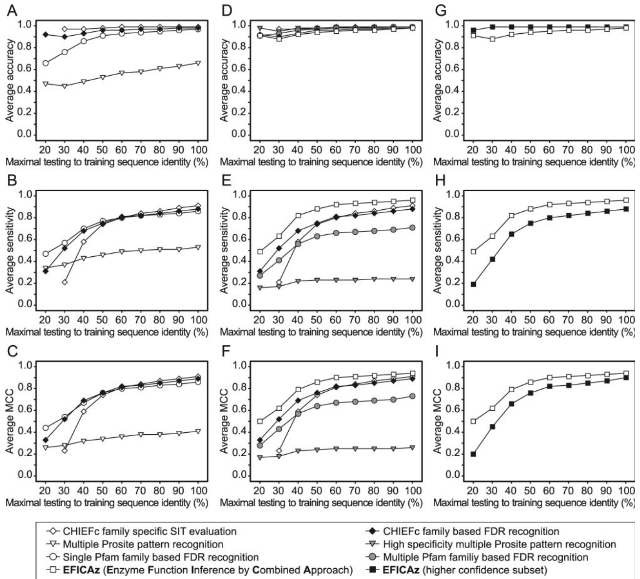
Figure 5. Benchmark of different enzyme function inference approaches by jackknife test. Accuracy (A, D, G), sensitivity (B, E, H) and Matthews Correlation Coefficient (C, F, I) values for different enzyme function inference methods, at different levels of maximal testing to training sequence identity, averaged per EC number. See Methods for a full description of the jackknife procedure. The plotted values are the averages of three repetitions of the jackknife analysis; the corresponding SDs are omitted for clarity, they range from 0.01 to 0.09, with a median value of 0.01.
