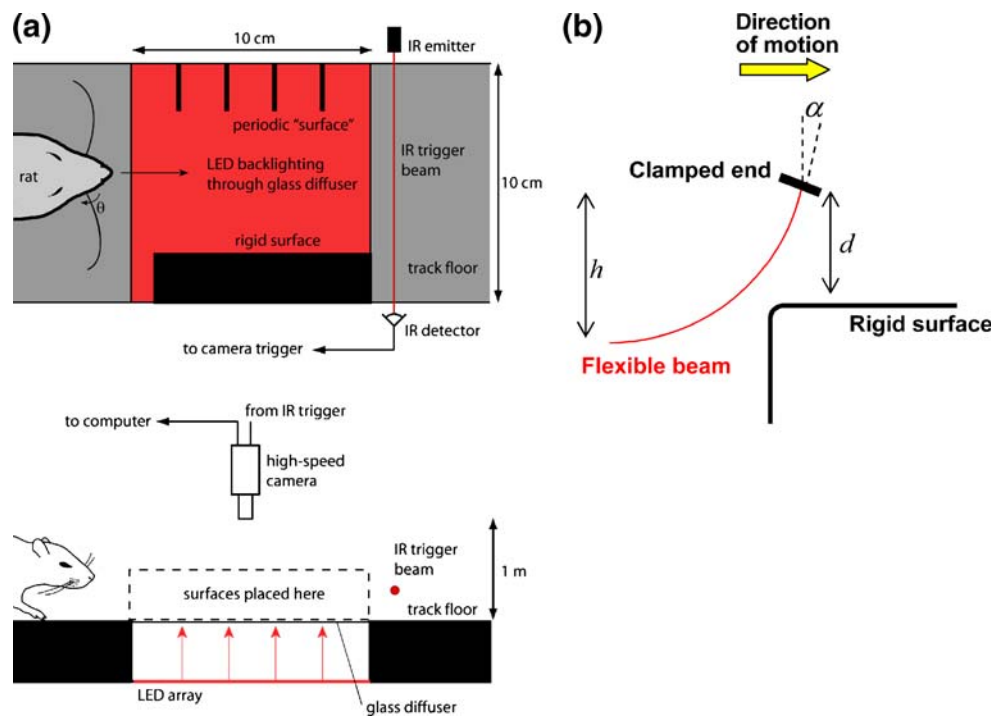
Fig. 1 Schematics of the experimental setup and computational model. (a) Top : Top view of track showing surfaces on either side, backlit image area, and IR trigger beam. Beam triggers camera to send buffered frames to computer after rat crosses image area. Bottom : Side view of track showing LED array and camera. (b) Schematic showing structure of the computational model and relevant parameters
